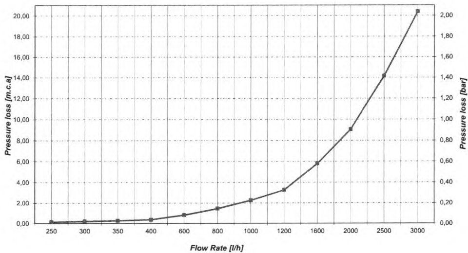
LAQUAS Q 3 1,6 DN20x115 (G 1" B)
