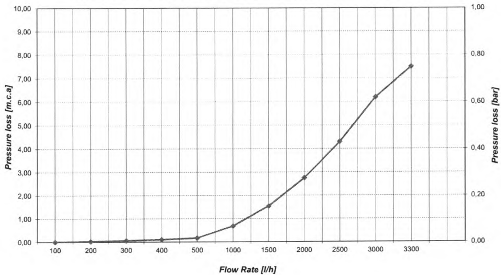
LAQUAM DN20x190 mm (G1" B) Q3=2.5 R100 - Pressure loss
